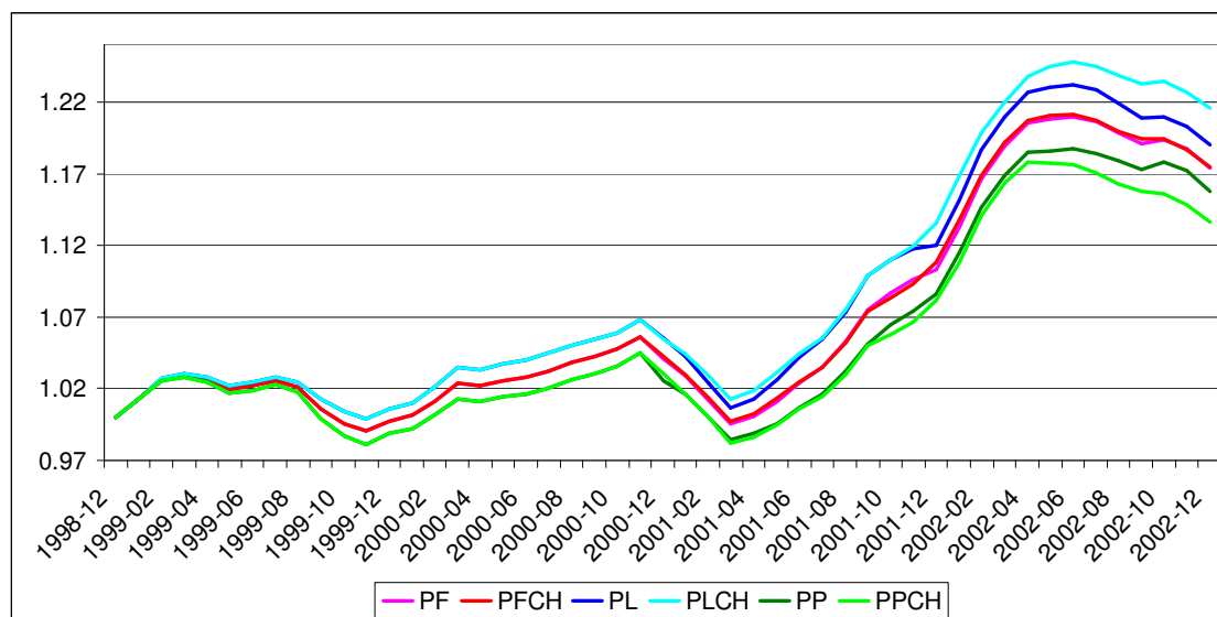
Chart 8: Rolling Year Mudgett Stone Fixed Base and Chained Fisher, Laspeyres and Paasche Price Indexes for Seven Kinds of Vegetables, 1998:12-2002:12
