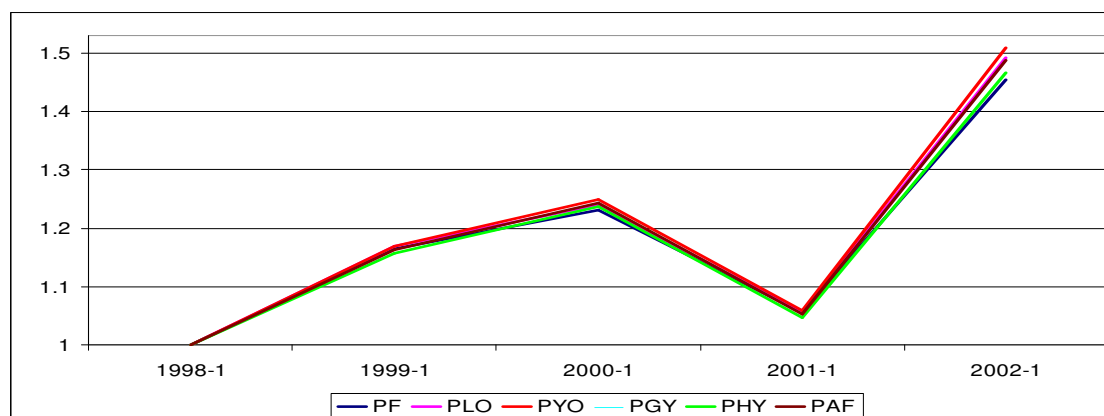
Chart 3: January 1998-2002 Year over Year Fisher, Lowe, Young, Geometric Young, Harmonic Young and Approximate Fisher Fixed Base Indexes
